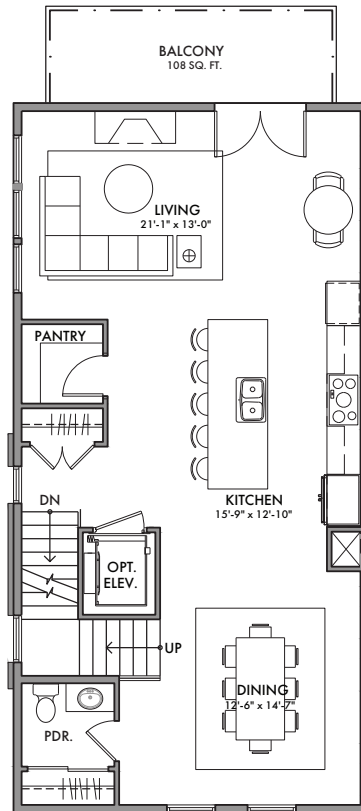
Main Living SECOND FLOOR CEILING: 9'-0"
