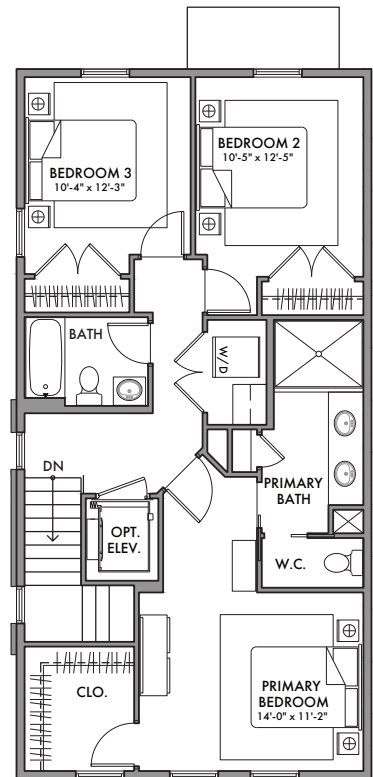
Bedrooms THIRD FLOOR CEILING: 9'-0"
