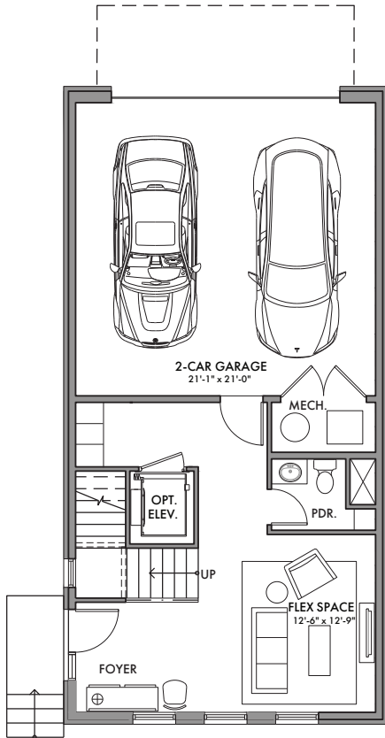
Entrance GROUND FLOOR CEILING: 9'-0"
