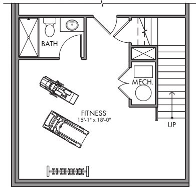
Alt. First Floor FITNESS ROOM CEILING: 9'-0"
