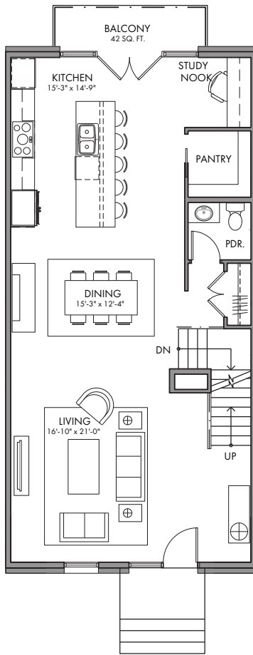
Main Living SECOND FLOOR CEILING: 9'-0"
