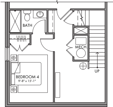
Alt. First Floor BEDROOM W/FULL BATH CEILING: 9'-0"
