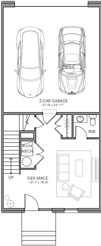
Entrance FIRST FLOOR CEILING: 9'-0"
