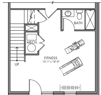
Alt. Ground Floor FITNESS CEILING: 9'-0"
