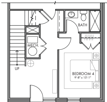
Alt. Ground Floor OPT. BEDROOM + FULL BATH CEILING: 9'-0"
