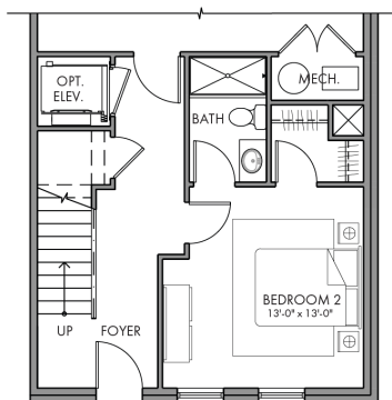
Alt. Ground Floor OPT. BEDROOM + FULL BATH CEILING: 9'-0"
