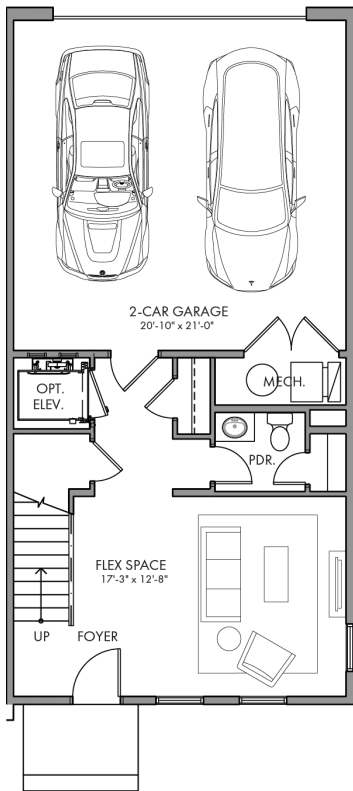
Entrance FIRST FLOOR CEILING: 9'-0"
